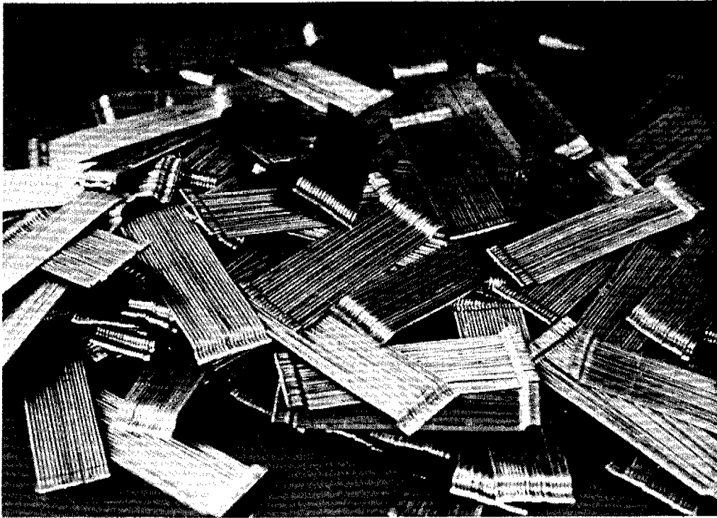
Figure 5 Glued bundles of steel fibres
