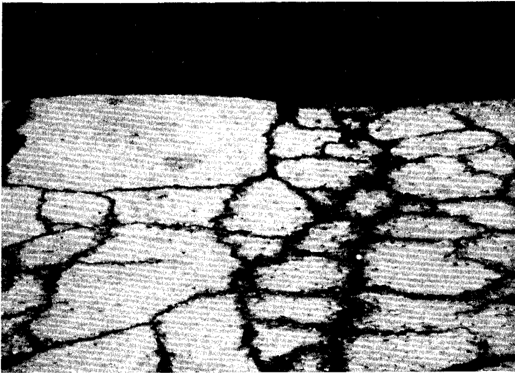
(a) Six months after resurfacing without using geotextiles
