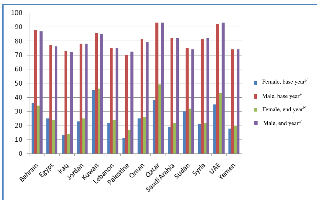
Figure I. Labour force participation rate, by gender
