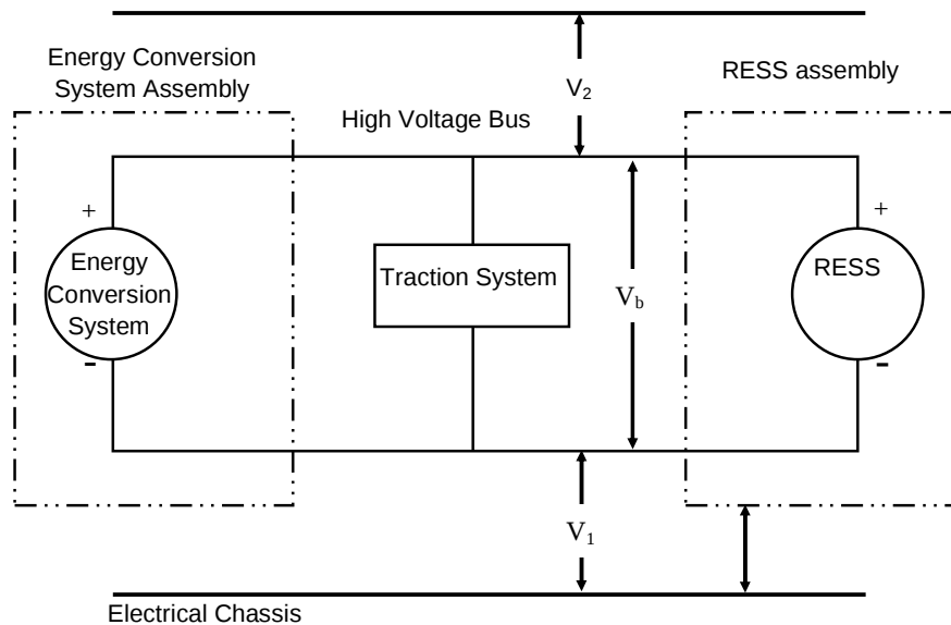
Measurement of V_b , V_1 , V_2
