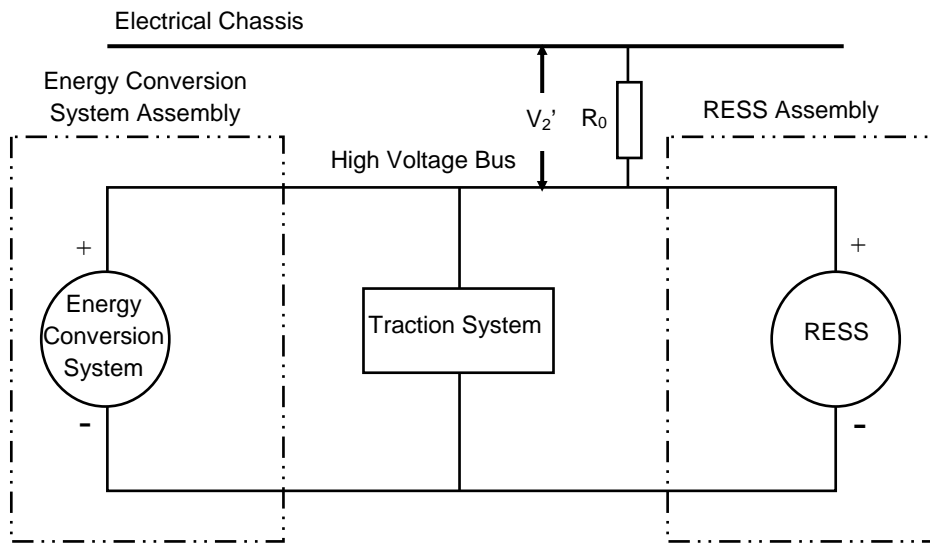
Figure 4: Measurement of V_2'
