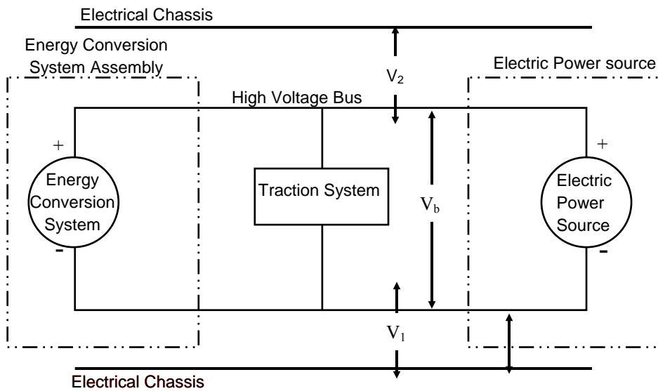
Figure 1 Measurement of V_b , V_1 , V_2
