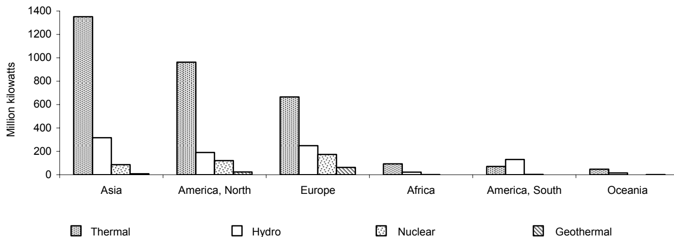
Figure 83: Net installed capacity of electric generating plants in 2007
