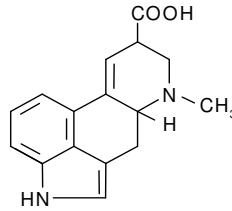
(8β)-9,10-didehydro-6-methylergoline-8-carboxylic acid
