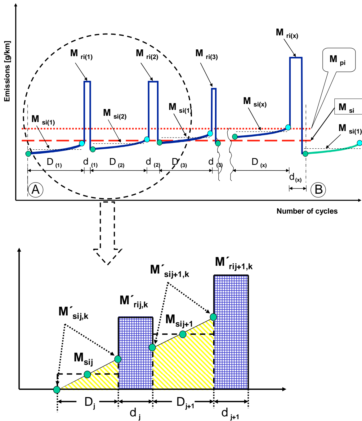
Figure 8/2: Parameters measured during emissions test during and between cycles where regeneration occurs (schematic example)
