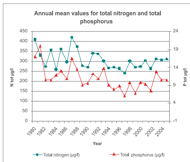
Annual mean values of total nitrogen and total phosphorus at the Oulankajoki station (Finland)
