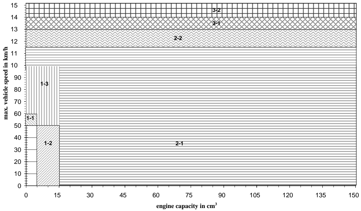
Figure 6-1: vehicle classification
