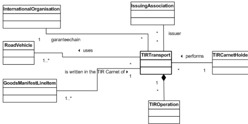
Figure 1.21 TIR transport class and its relationships
