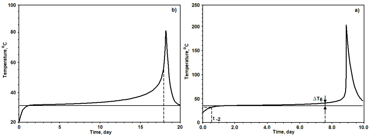
Fig. 2. Determining SADT along the H1 test: the autocatalytic reaction, lumped system. (a) – the ambient temperature equals SADT (H1 test); (b) - the ambient temperature equals the critical temperature of thermal explosion .
