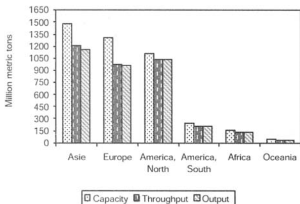
Refinery distillation capacity, troughput and output 2002
