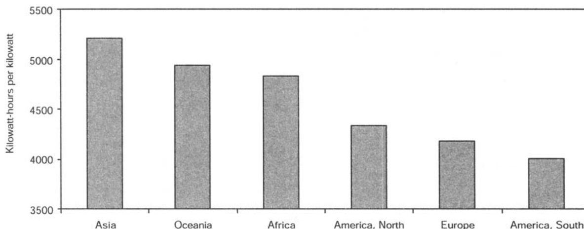
Estimated total utilization of installed electric generating capacity in 2002
