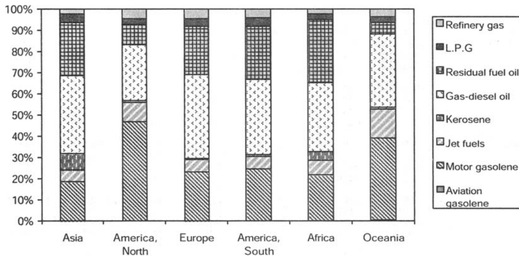
World production of energy products from refineries 2002
