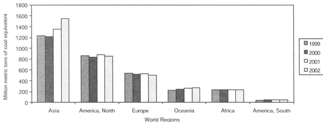
Production of solid fuels by world regions 1999-2002
