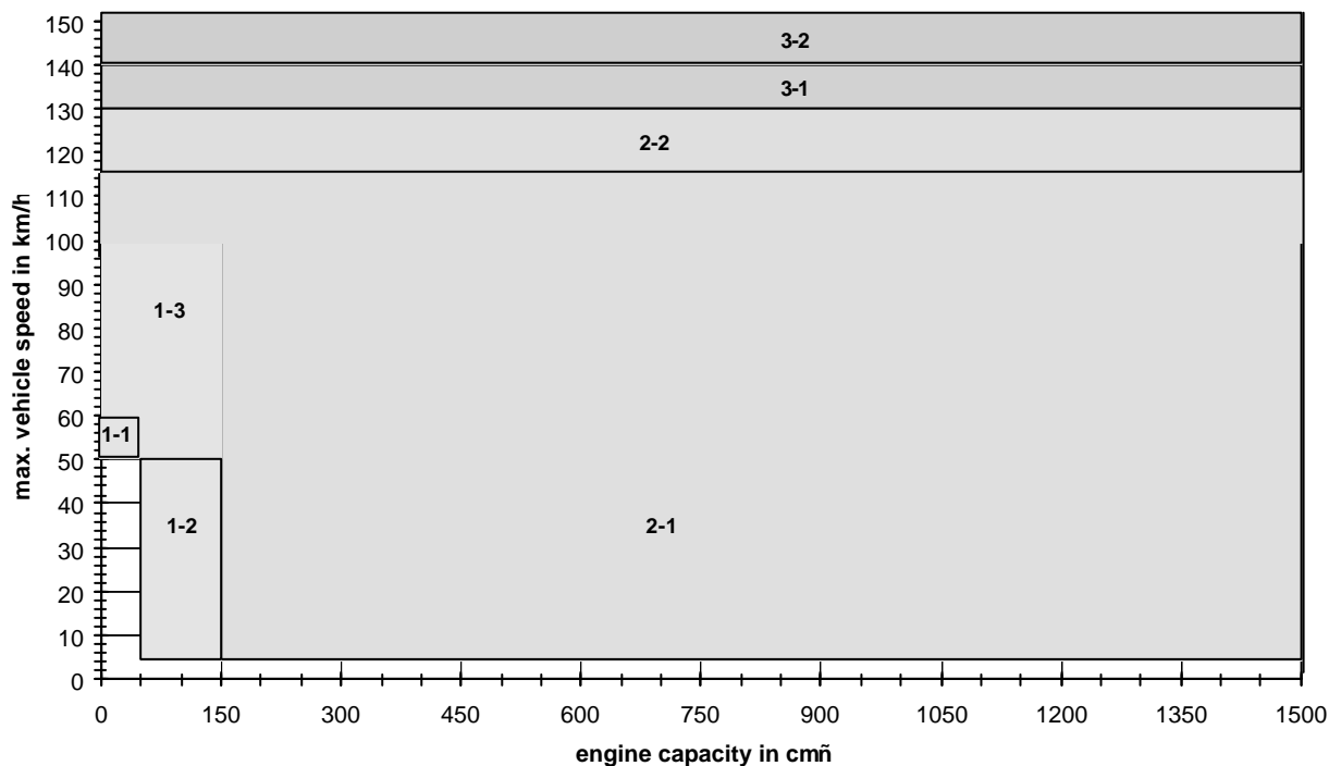
Figure 6-1: vehicle classification
