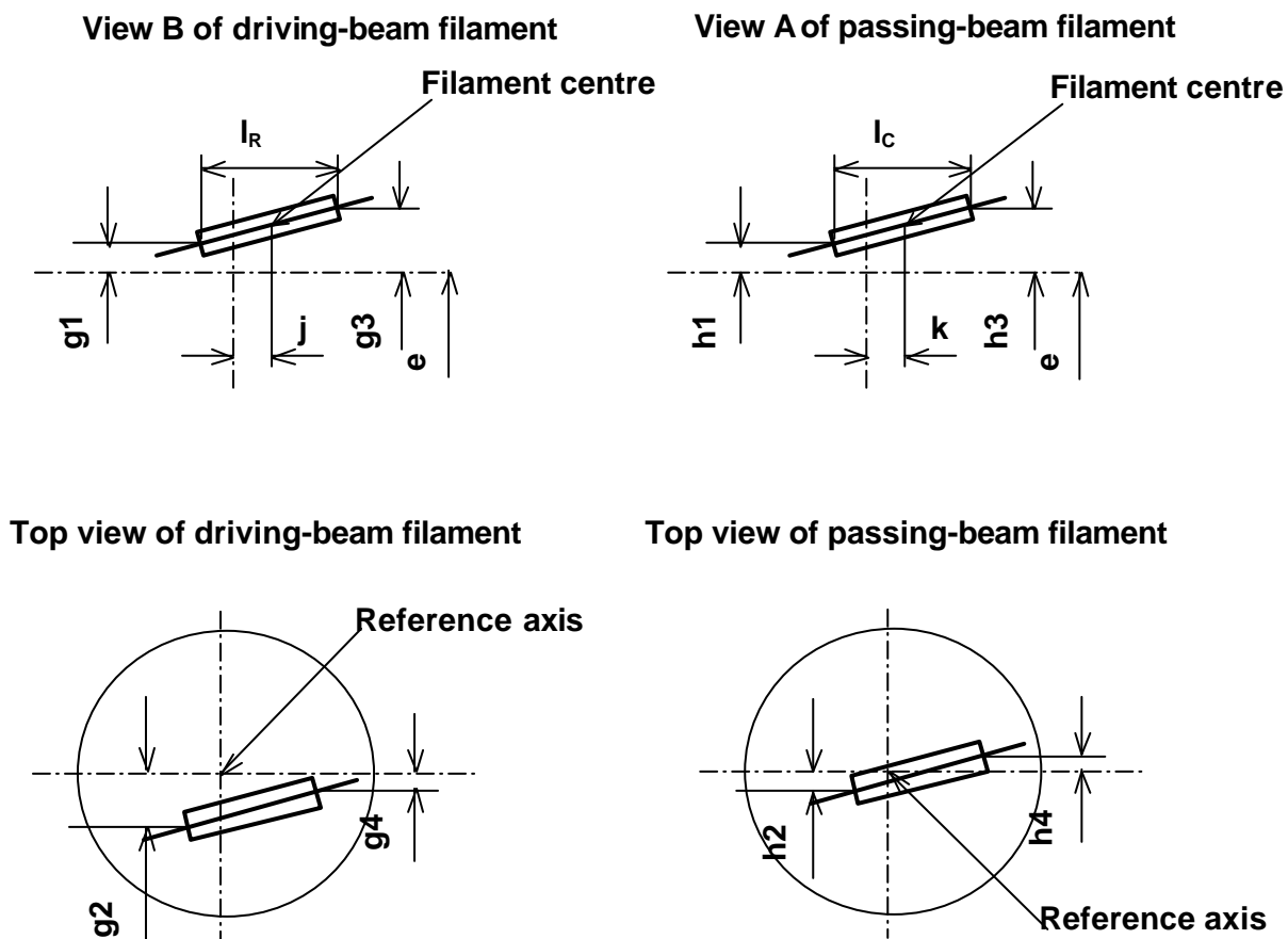
Figure 3 Filament position and dimensions
