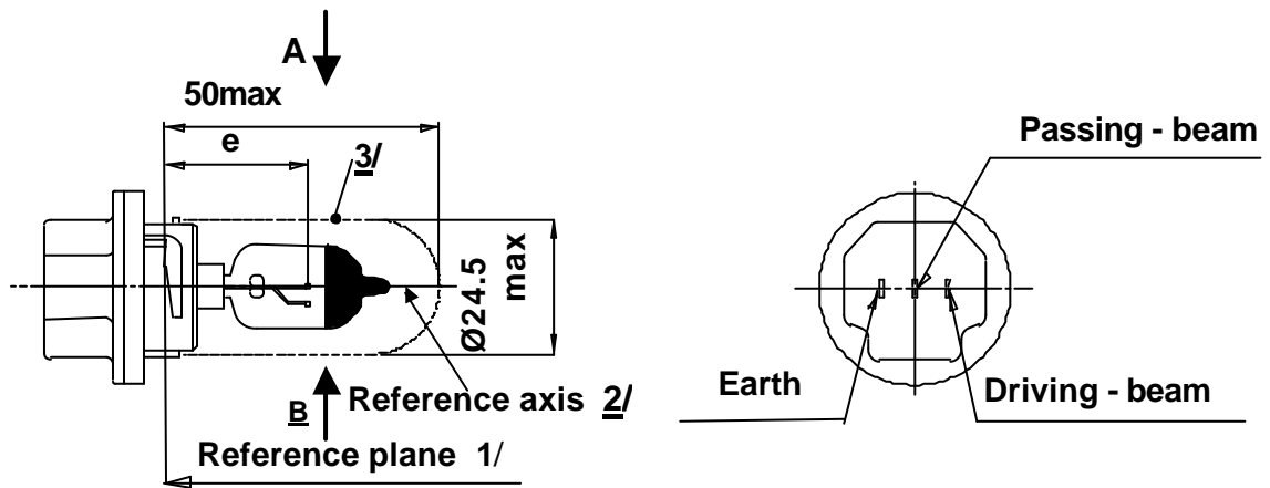
Figure 1 Main drawing
