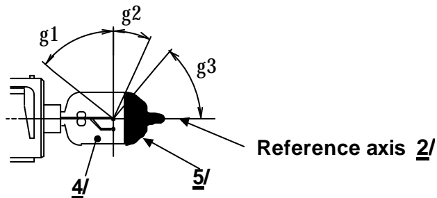
Figure 2 Distortion free area 4/ and black top 5/
