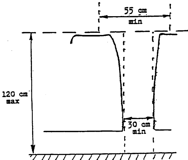
Figure 20 Determination of unobstructed access to door (See paragraph 5.7.1.10.2.)
