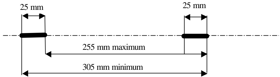
Figure 4: Distance between both low anchorage zones
