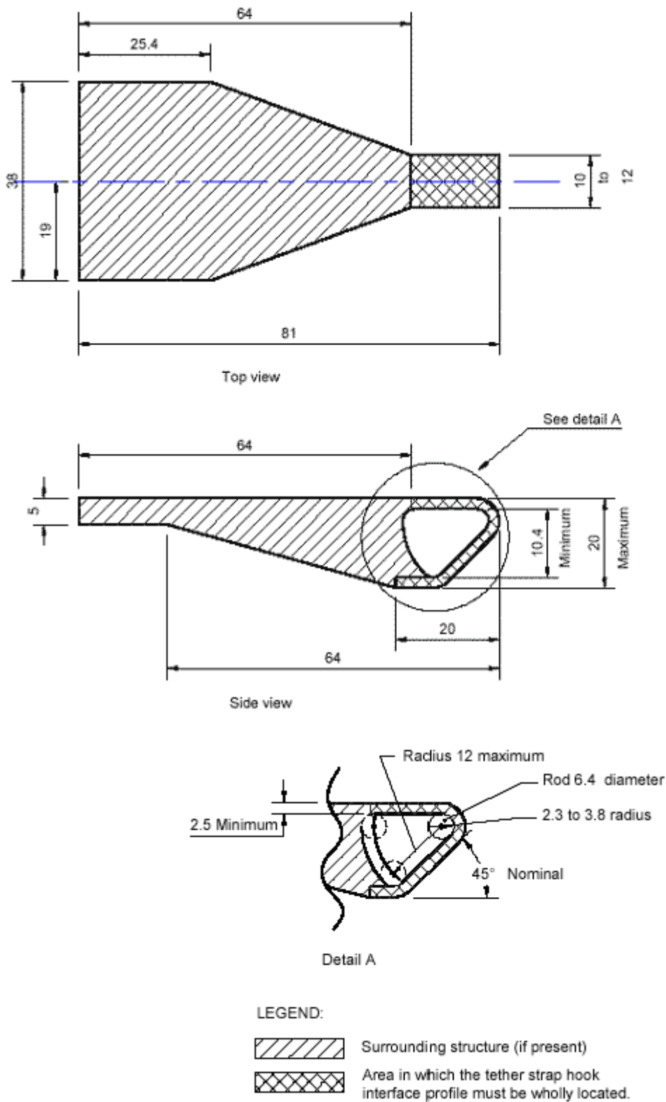
Figure 3: ISOFIX Top tether connector (hook type) dimensions
