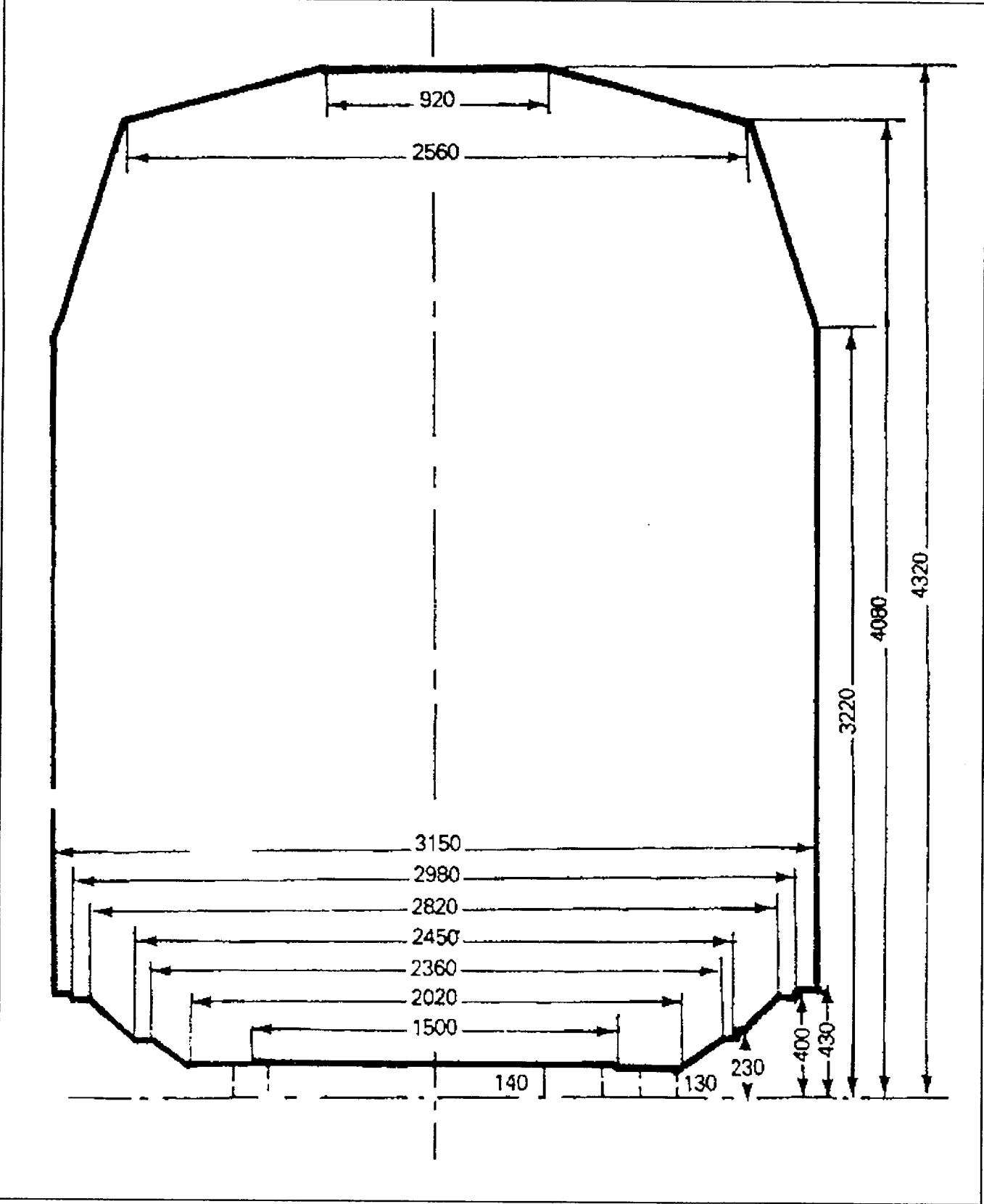
Figure I. UIC Loading gauge specifications UIC/B
