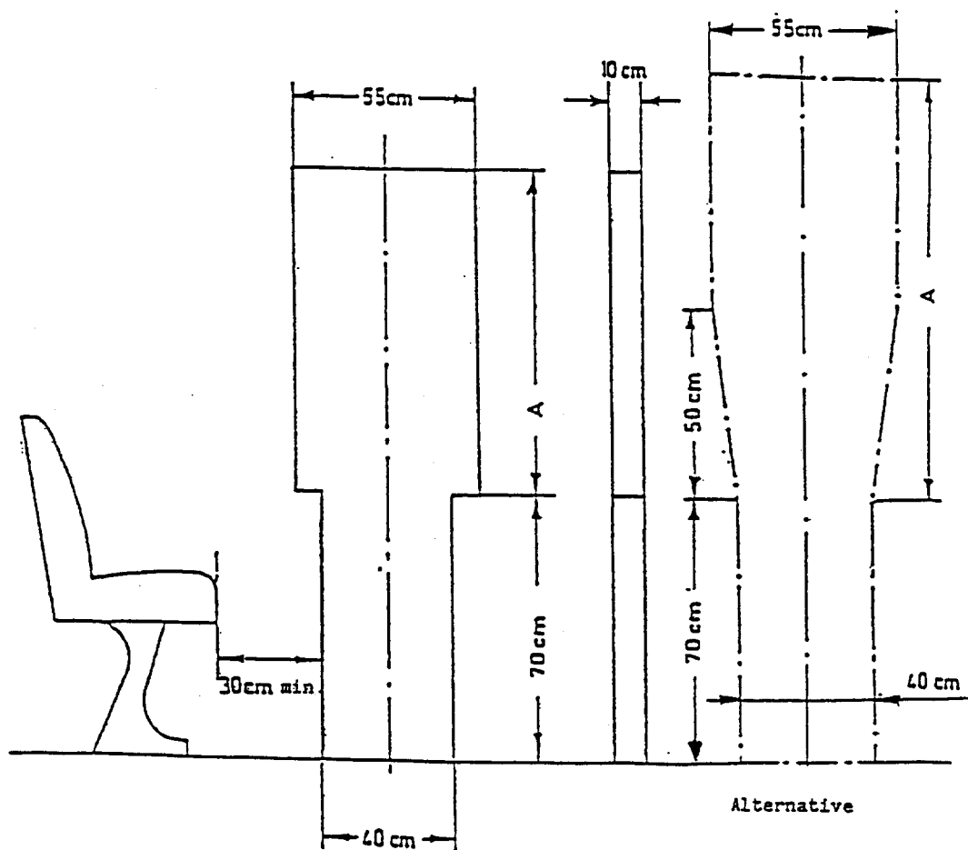
Figure 1 ACCESS TO SERVICE DOORS (see paragraph 5.7.1.)
