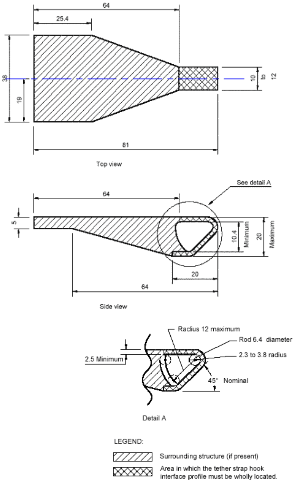
Figure 3: ISOFIX Top tether connector (hook type) dimensions
