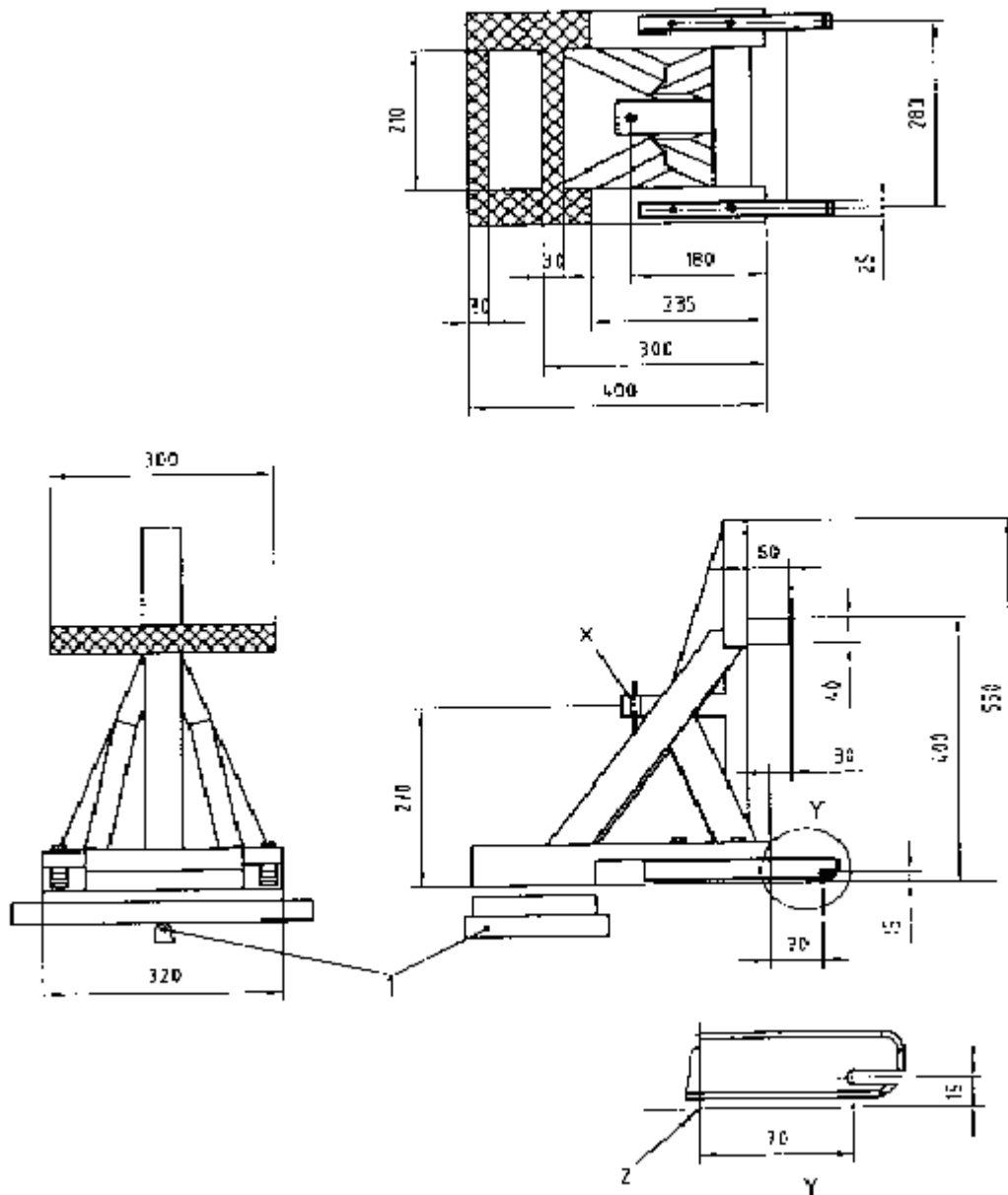
Figure 2: Static force application device (S-FAD), dimensions
