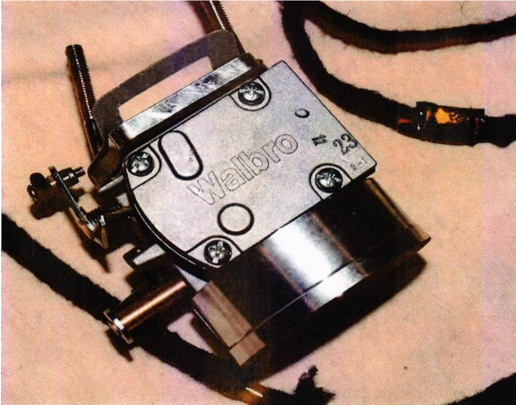
- Parts from a large suicide drone bearing "Walbro 23".
