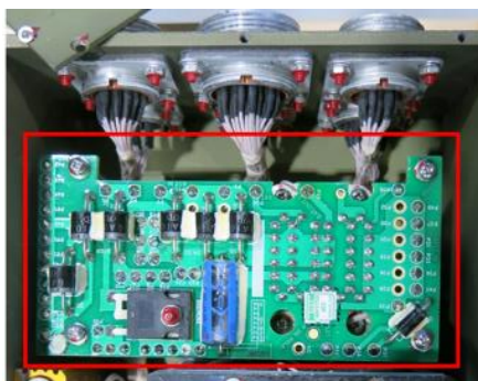
Figure 51.41. Battery box seized by the UK in 2022
