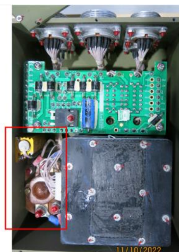
Figure 51.39. Battery box seized by the UK in 2022
