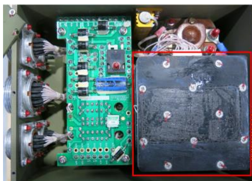
Figure 51.44. Battery box seized by the UK in 2022
