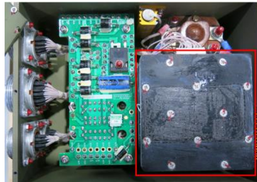
Figure 51.44. Battery box seized by the UK in 2022
