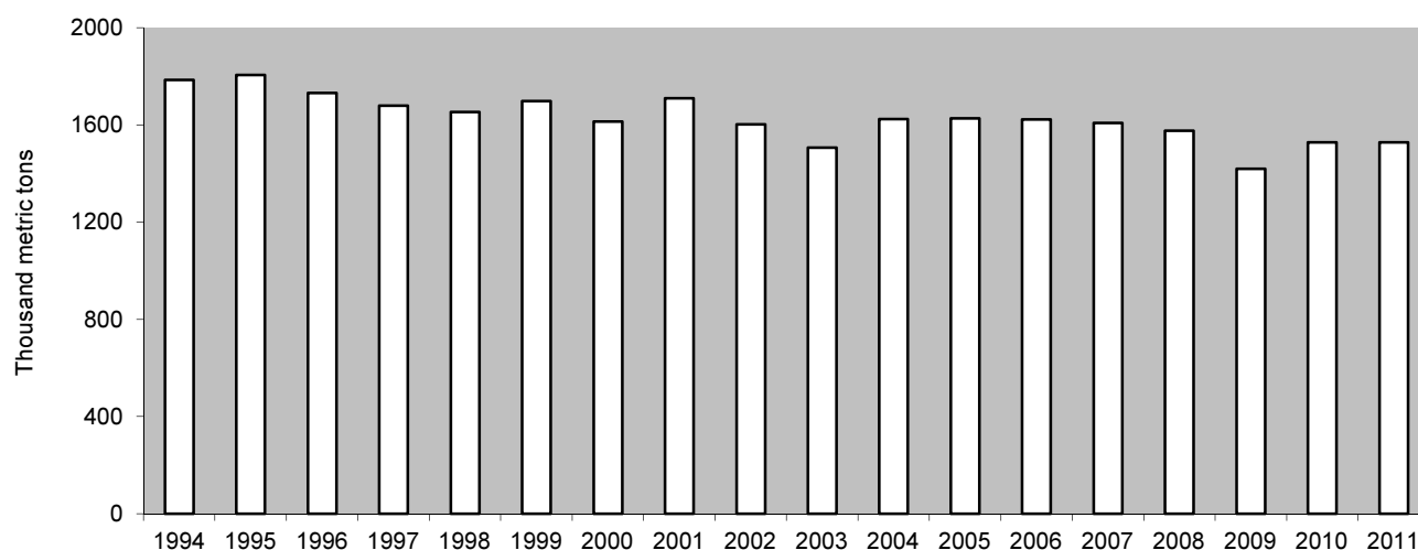
Figure 49: World production of aviation gasoline 1994-2011
