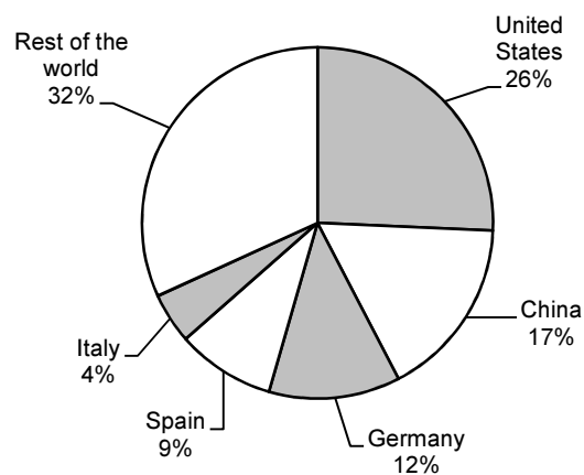
Figure 88: Major Other electricity producing countries in 2011
