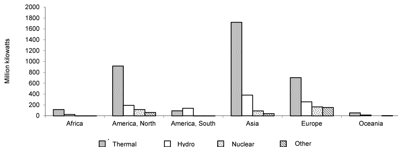
Figure 81: Net installed capacity of electric generating plants, by region, in 2011
