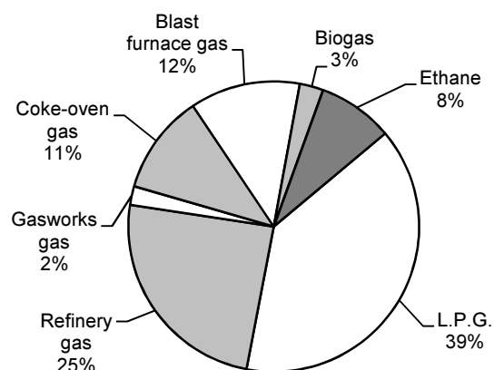
Figure 78: World production of other gases in 2011
