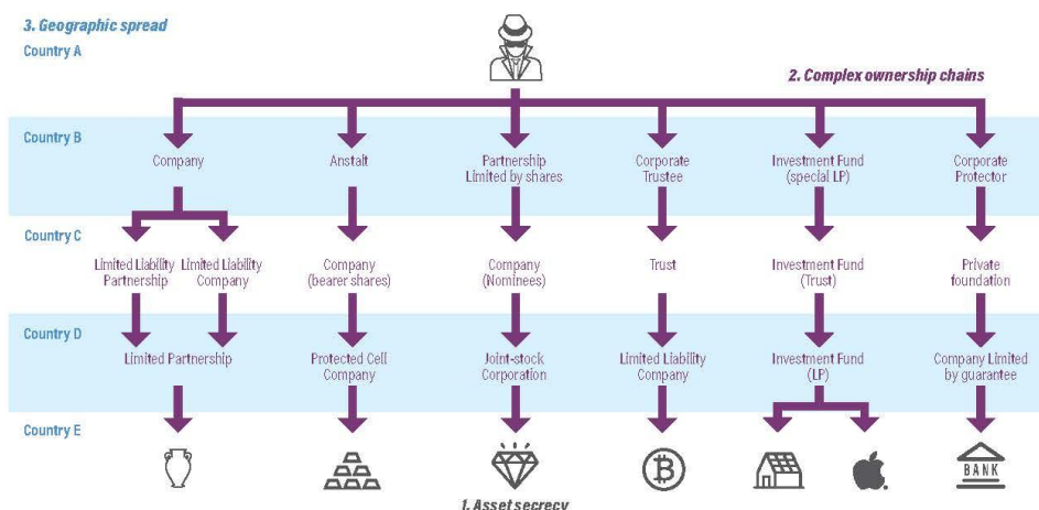
FIGURE 1: SCHEMATIC DIAGRAM OF THREE TYPES OF SECRECY
