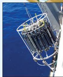
© Digna Rueda CTD sensor equipped with water sampling rosette deployed at the BATS station.
