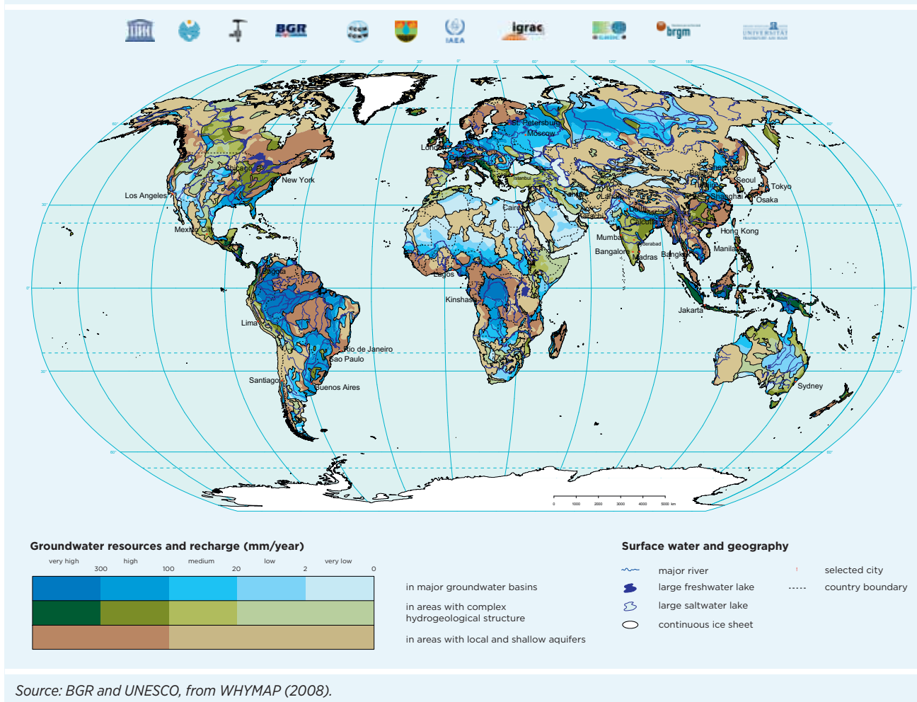
Groundwater resources of the world
