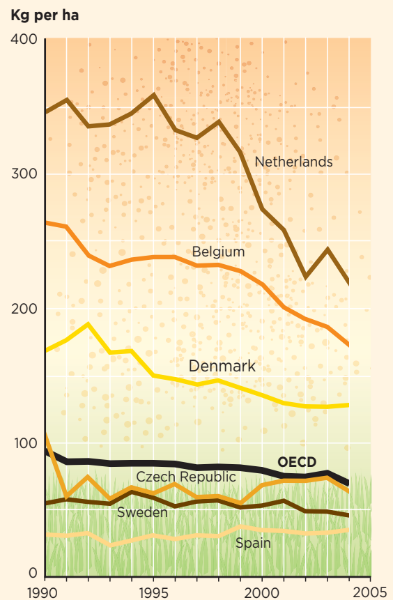
FIGURE 4.2 Nitrogen balance in Europe
