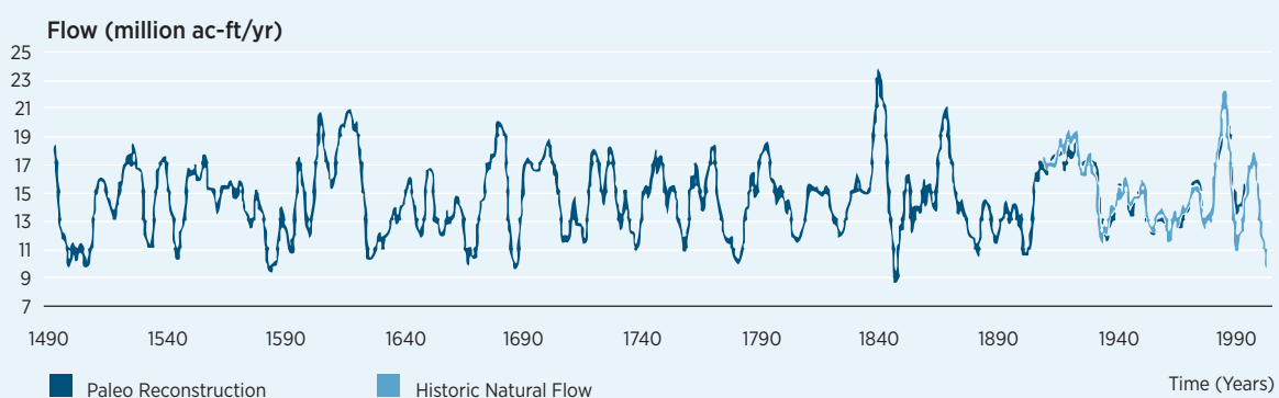
Paleo reconstruction of the Colorado River streamflow
