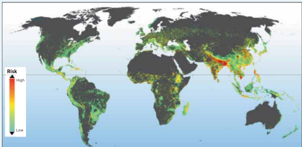
Hazard mortality risk (floods, tropical cyclones and precipitation-triggered landslides)
