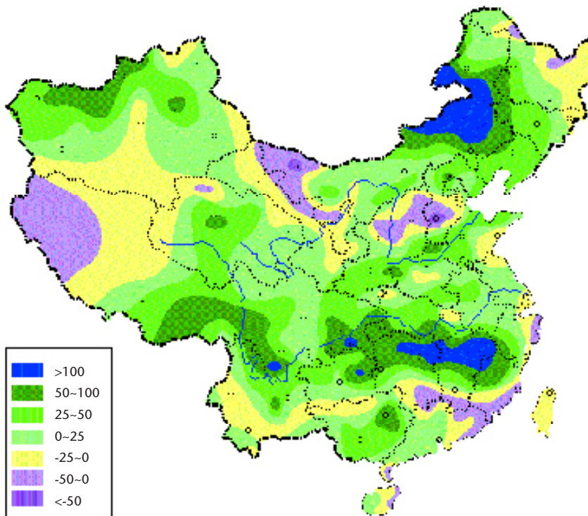
Figure 6. Significant climate anomalies and episodic events of 1998.
