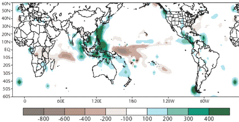
Figure 5. Precipitation anomalies for October 1998 to December 1998. Anomalies are departures from the 1979-95 base-period means. Data were obtained from a merge of rain gauge observations and satellite derived precipitation estimates. The satellite estimates were generated by the outgoing long-wave radiation precipitation index (OPI) technique (Xie and Arkin, 1997) which were merged with rain gauge data via the method adopted from Xie and Arkin (1996). (Source: CPC, NOAA)
