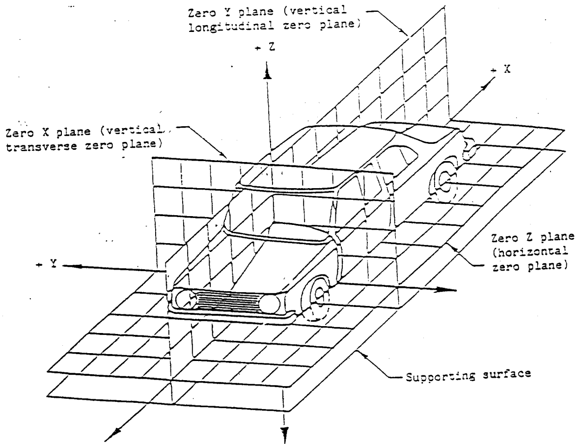
Figure - Three-dimensional reference system
