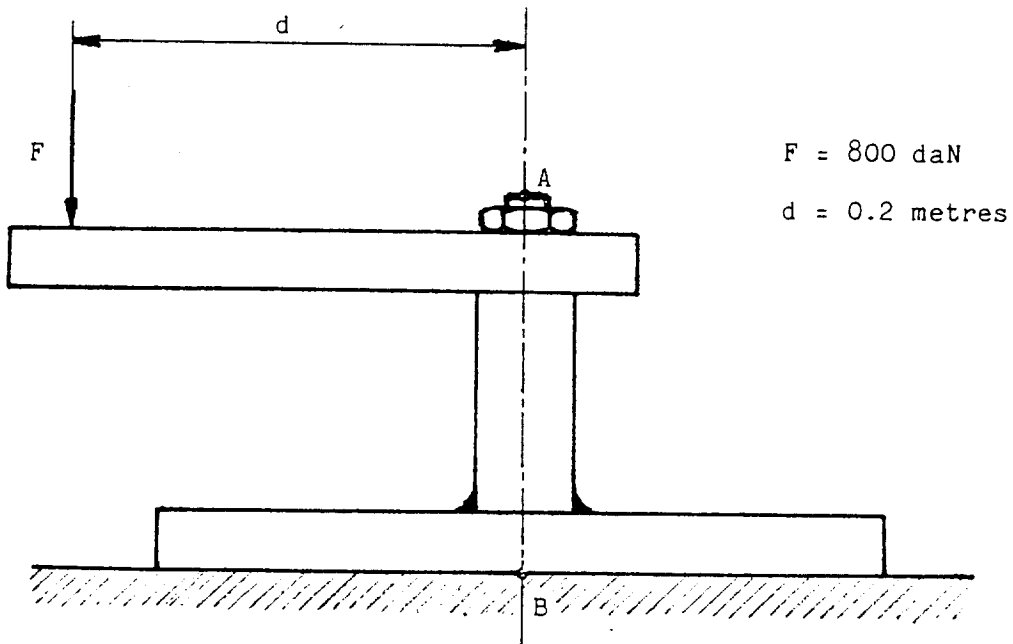
Fig. 1 b Measurement of the testing set-up rigidity
