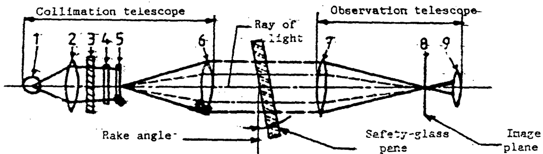
Figure 12 : Arrangement of apparatus
