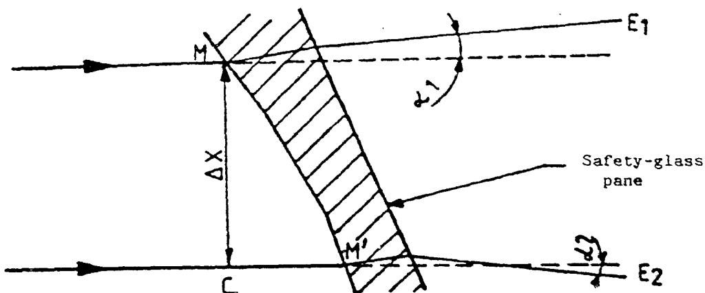
Figure 6 : Diagrammatic representation of optical distortion
