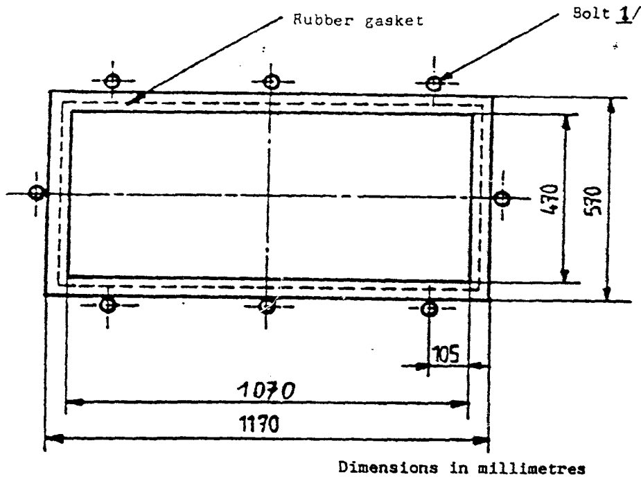
Figure 3 : Support for headform tests
