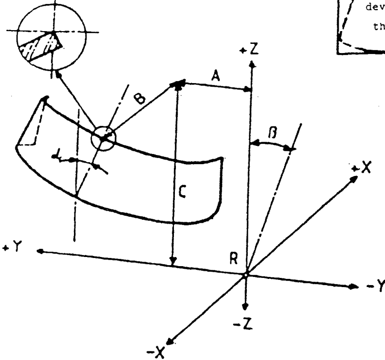
R-point co-ordinates relative to the windscreen
