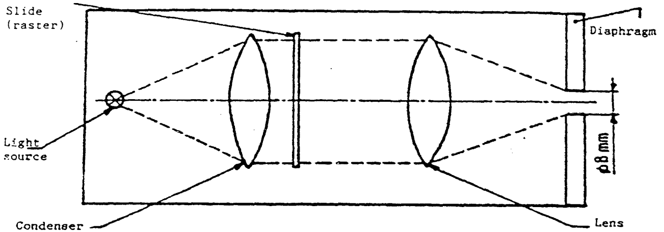
Figure 7 : Optical arrangement of the projector
