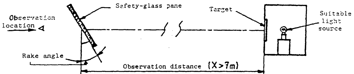
Figure 12 : Arrangement of apparatus
