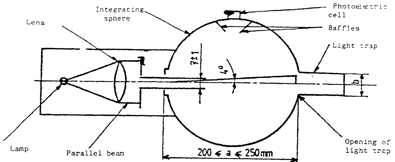
Figure 5 : Hazemeter
