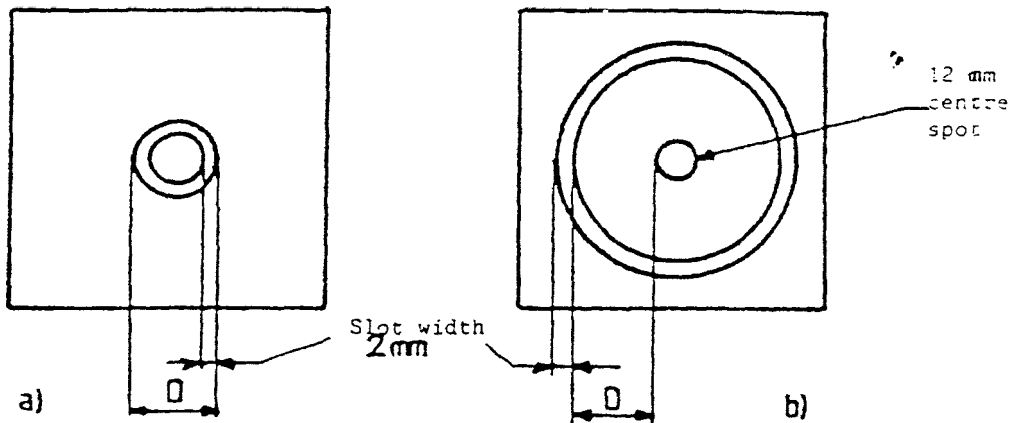
Figure 11 : Dimensions of targets
