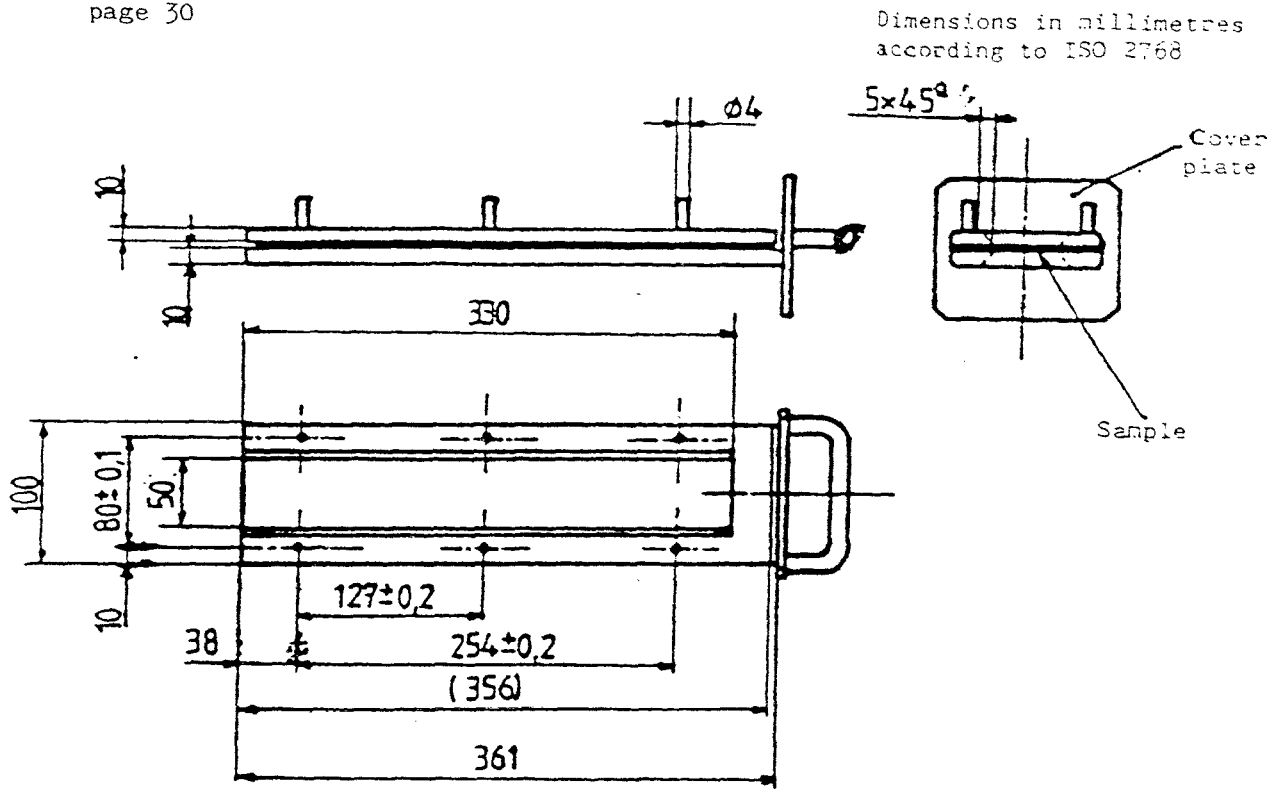
Figure 18 : Example of sample holder
