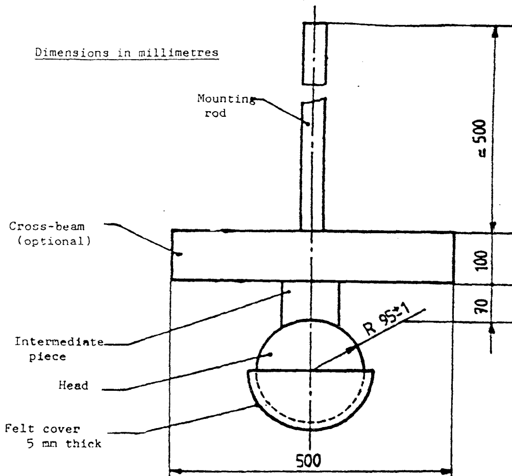
Figure 2 : Headform weight
