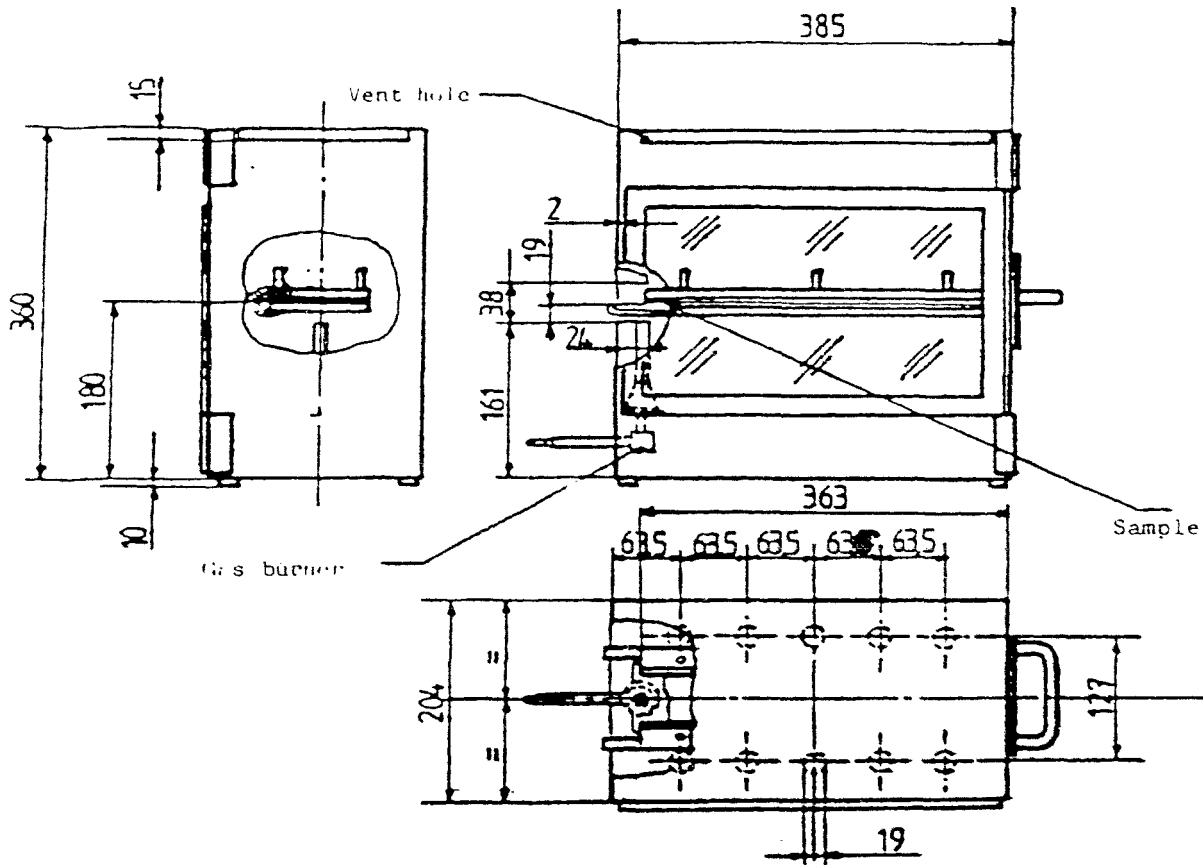
Figure 16 : Example of combustion chamber
