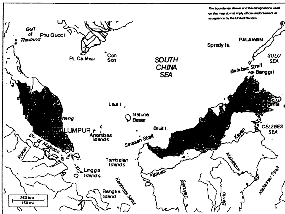
Figure 1. Regional drainage pattern and major surface water features of Malaysia
