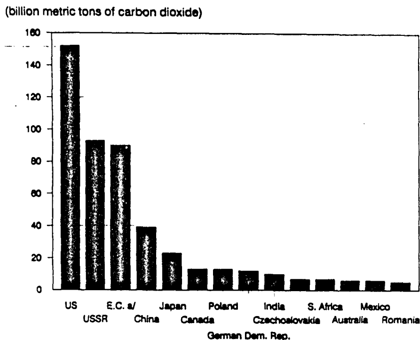
Figure XIII.2. Cumulative emissions of carbon dioxide from fossil fuels in 25 countries with the highest emissions, 1950-1989
