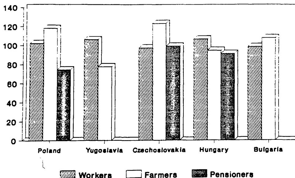
Figure VII.6. Relative per capita income in 1989 in selected Eastern European countries
