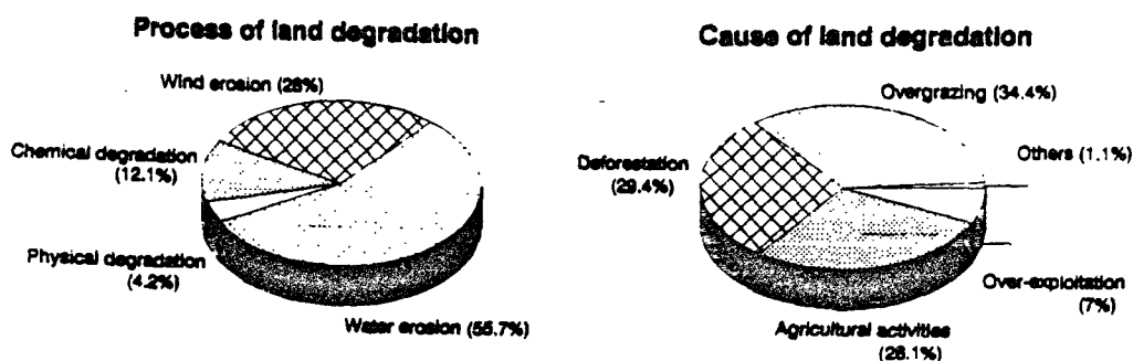
Figure XIII.8. Land degradation processes and causes
