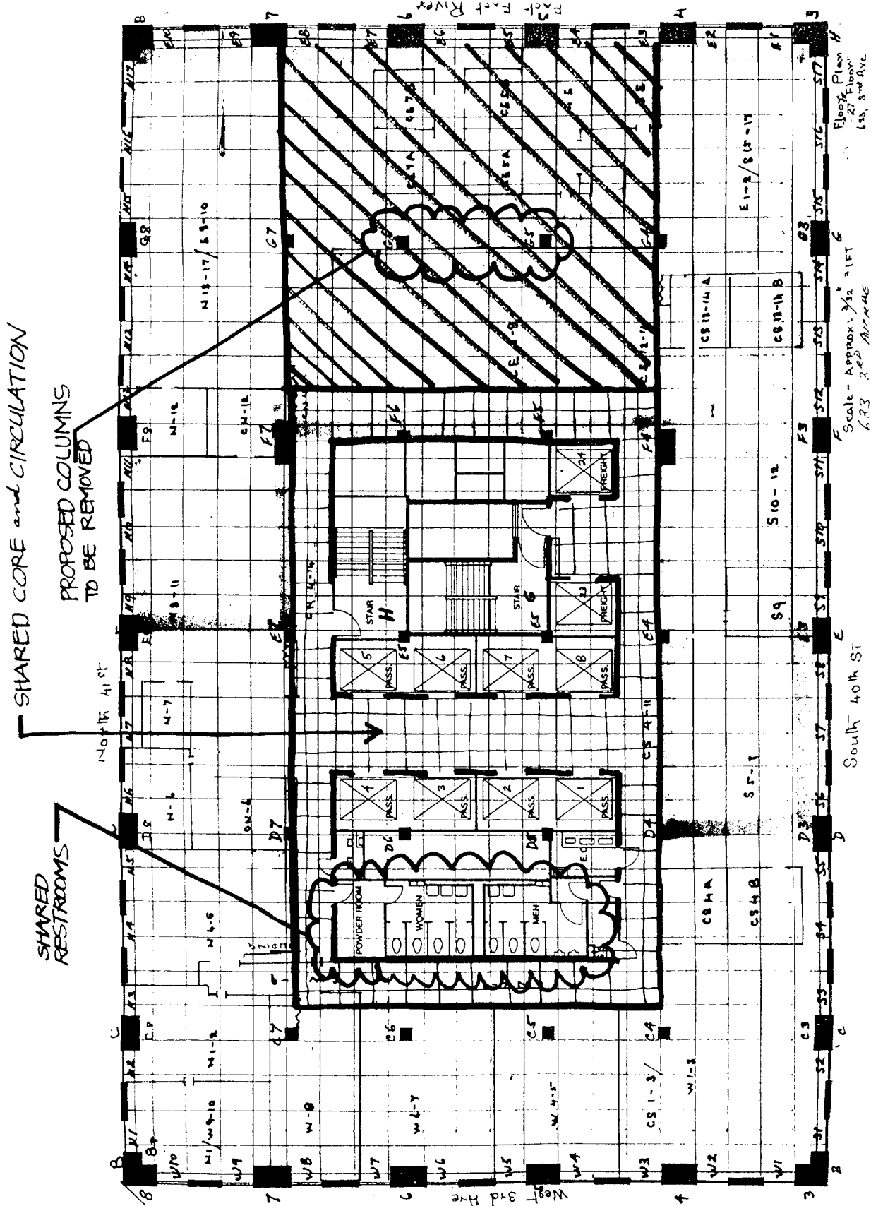
Figure II. Proposed layout of the twenty-seventh floor at 633 Third Avenue
