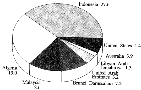
Figure V.7. International trade by LNG tankers in 1990 Billion cubic meters
