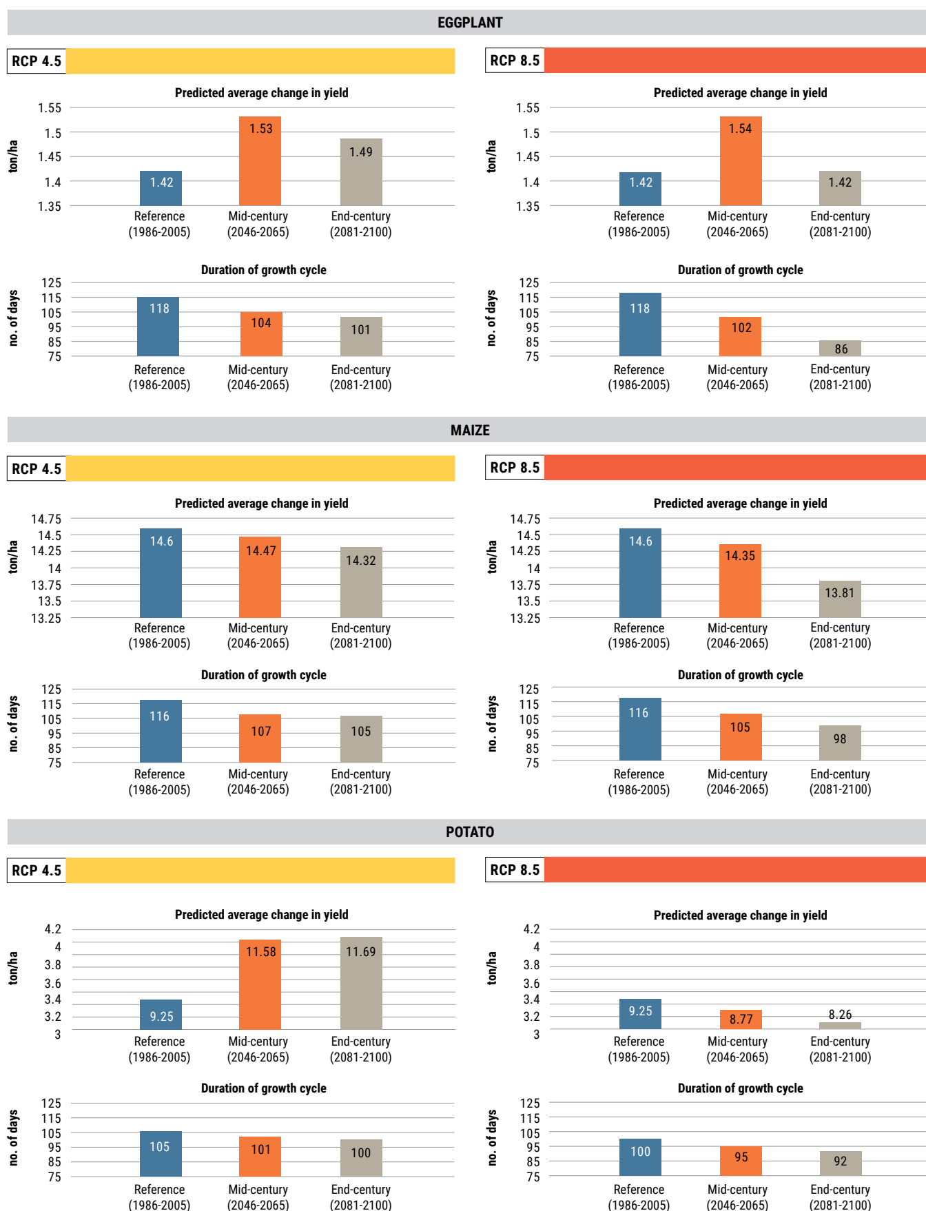
FIGURE 99: Simulated yield and growing-period duration of eggplant, maize and potato for the reference period, mid-century and end-century for RCP 4.5 and RCP 8.5 in Lebanon
