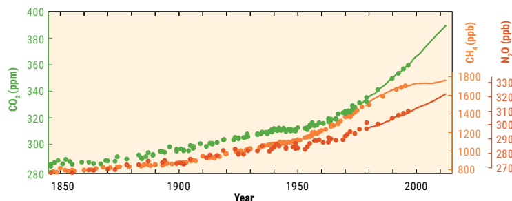
FIGURE 7: Globally averaged observed greenhouse gas concentrations until 2011
