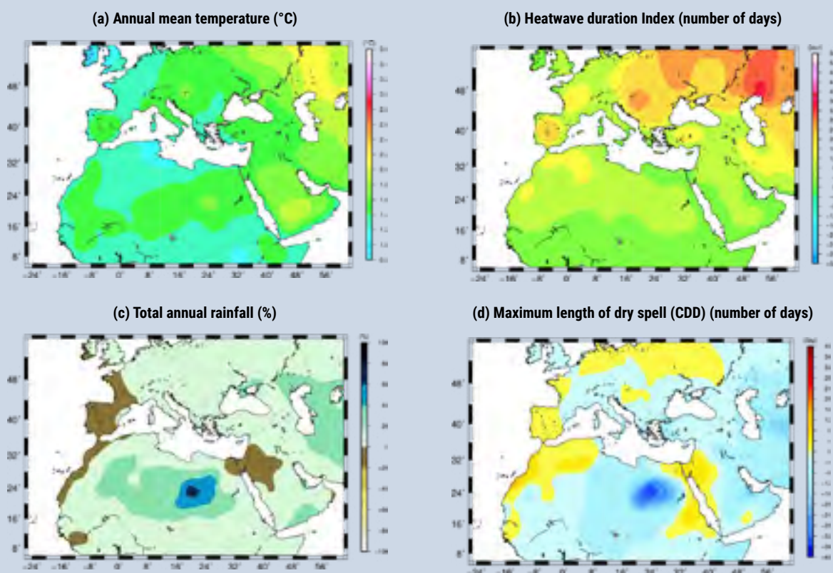
FIGURE 41: Future changes in different variables from ALADIN-Climate projections for RCP 8.5 for the future period 2036–2065 compared to the reference period 1971–2000
