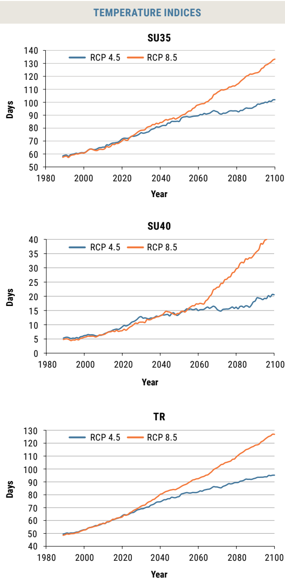
FIGURE 76: Mean change in selected extreme events indices over time for ensemble of three RCP 4.5 and RCP 8.5 projections for the Nahr el Kabir River basin
