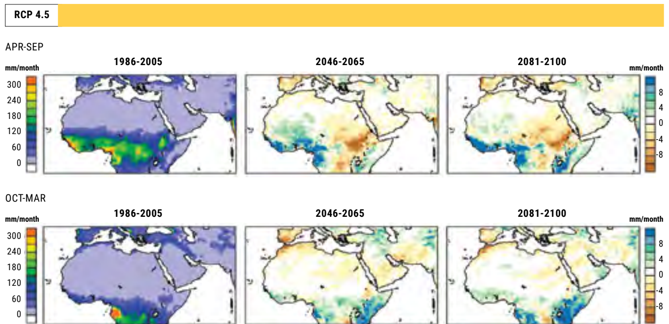
FIGURE 22: Mean change in seasonal precipitation for mid- and end-century for ensemble of three RCP 4.5 projections compared to the reference period
