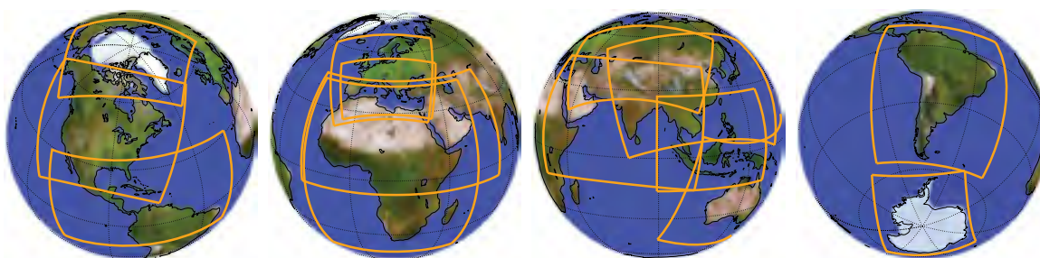
FIGURE 15: CORDEX domains
