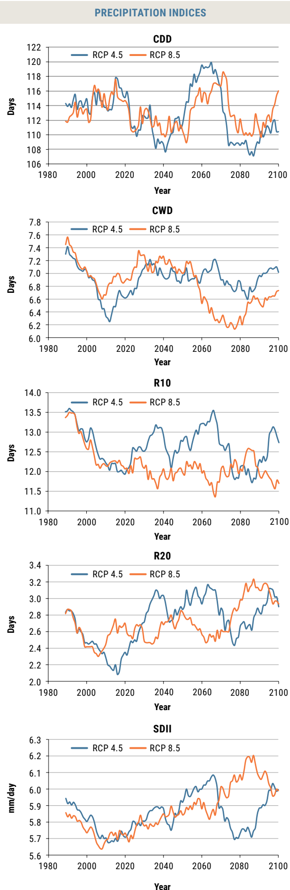
FIGURE 76: Mean change in selected extreme events indices over time for ensemble of three RCP 4.5 and RCP 8.5 projections for the Nahr el Kabir River basin
