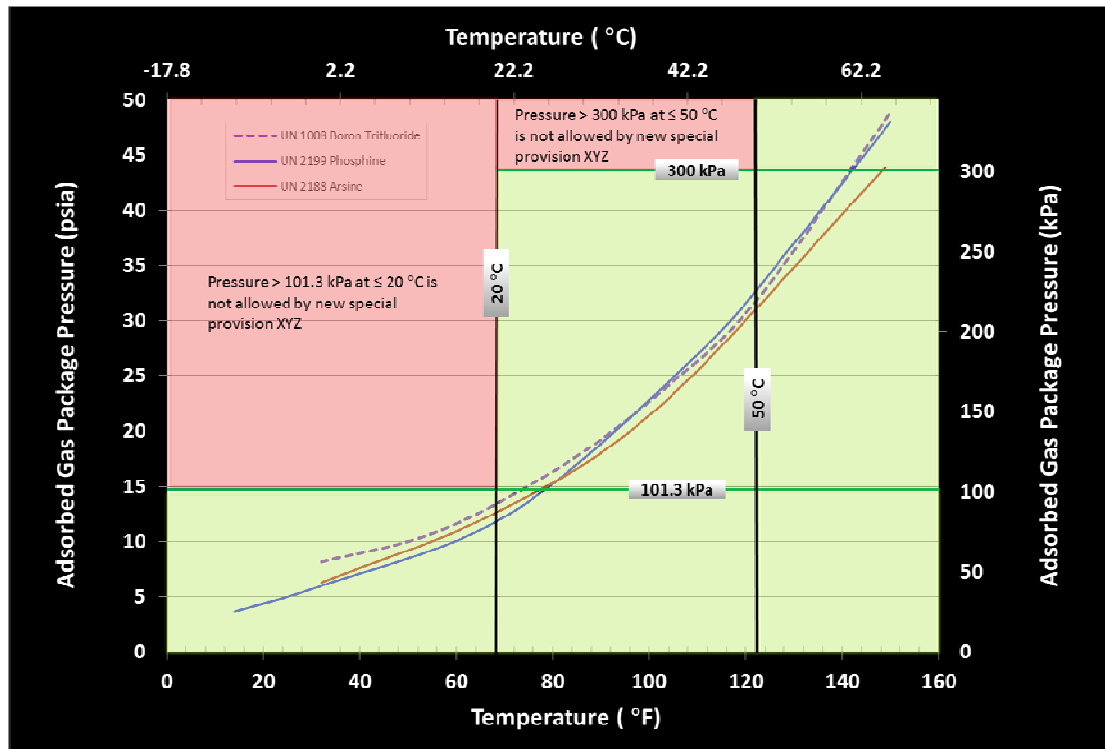
Figure 1—Adsorbed Gas Package Pressure as a Function of Temperature
