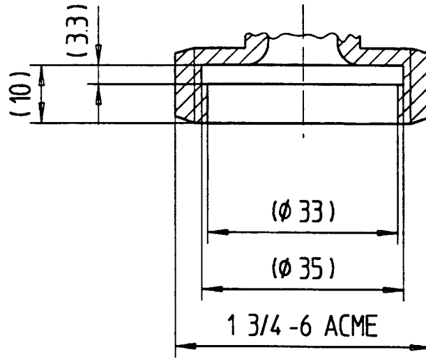
Figure 4 Connecting area of the ACME filling unit
