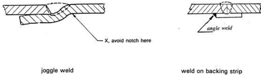
Figure 2 Circumferential butt weld
