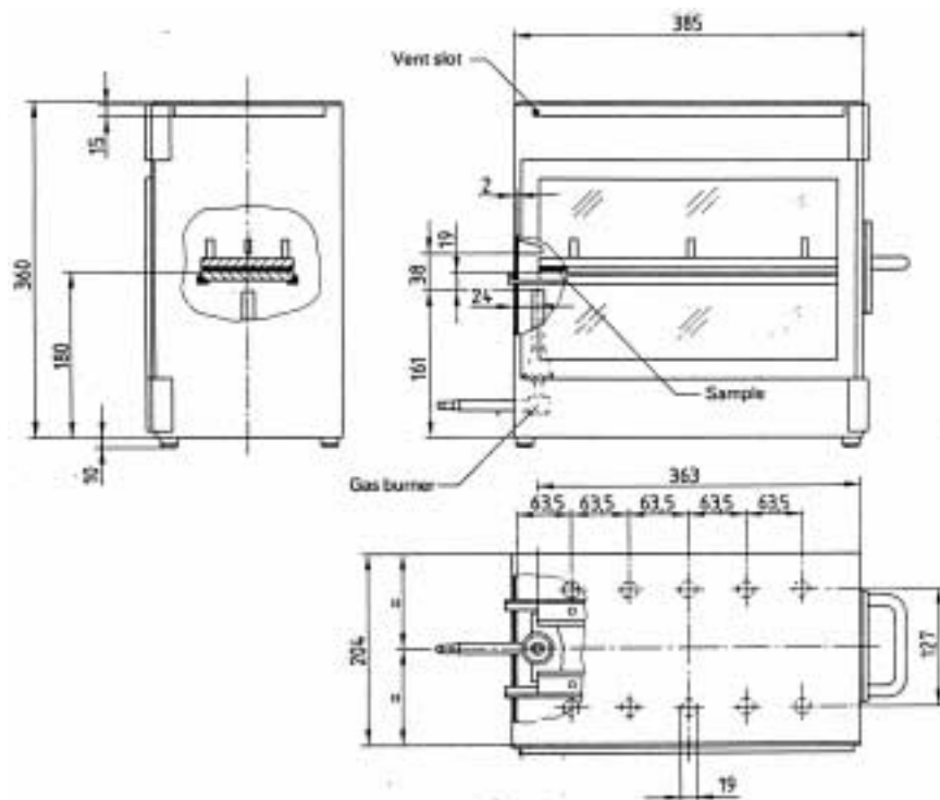
Figure 2 Example of combustion chamber (Dimensions in millimetres)
