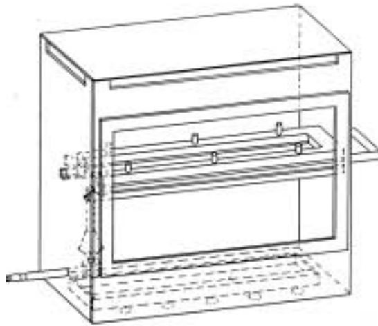
Figure 1 Example of combustion chamber with sample holder and drip tray
